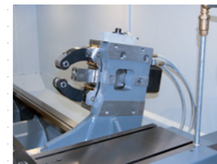
Self-centering follower rest, hydraulically actuated
