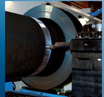
Cylinder machining
