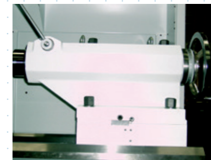
Heavy-duty tailstock with 140 mm quill diameter (E80 only)
