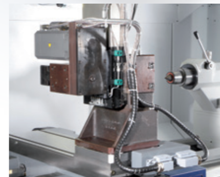
200 mm stroke Y-axis (only with E110/E120)
