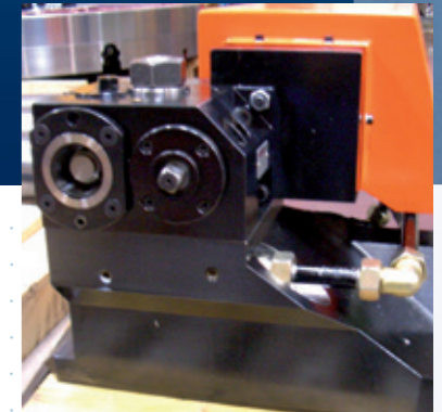
Tool holder head for driven tools, Capto C8 holding fixture
